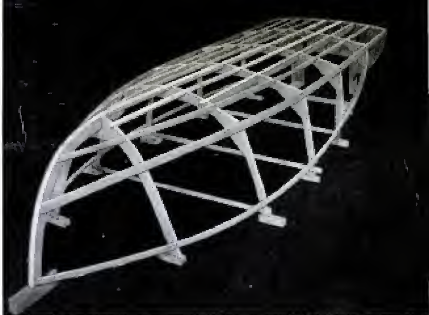
Some boat kits are assembled directly on floor. Unless floor is level, frames and stem must be leveled with blocks, above
